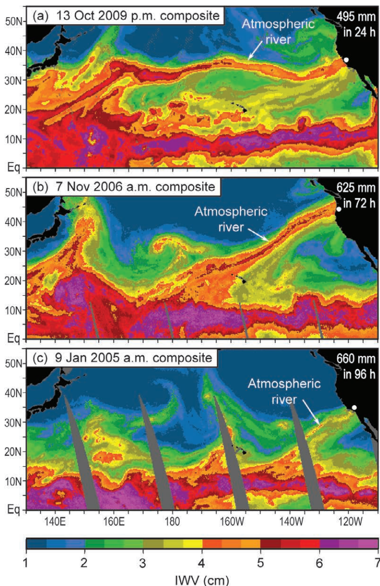
FIG. 4. Examples of atmospheric river events (from Ralph et al. 2011).
