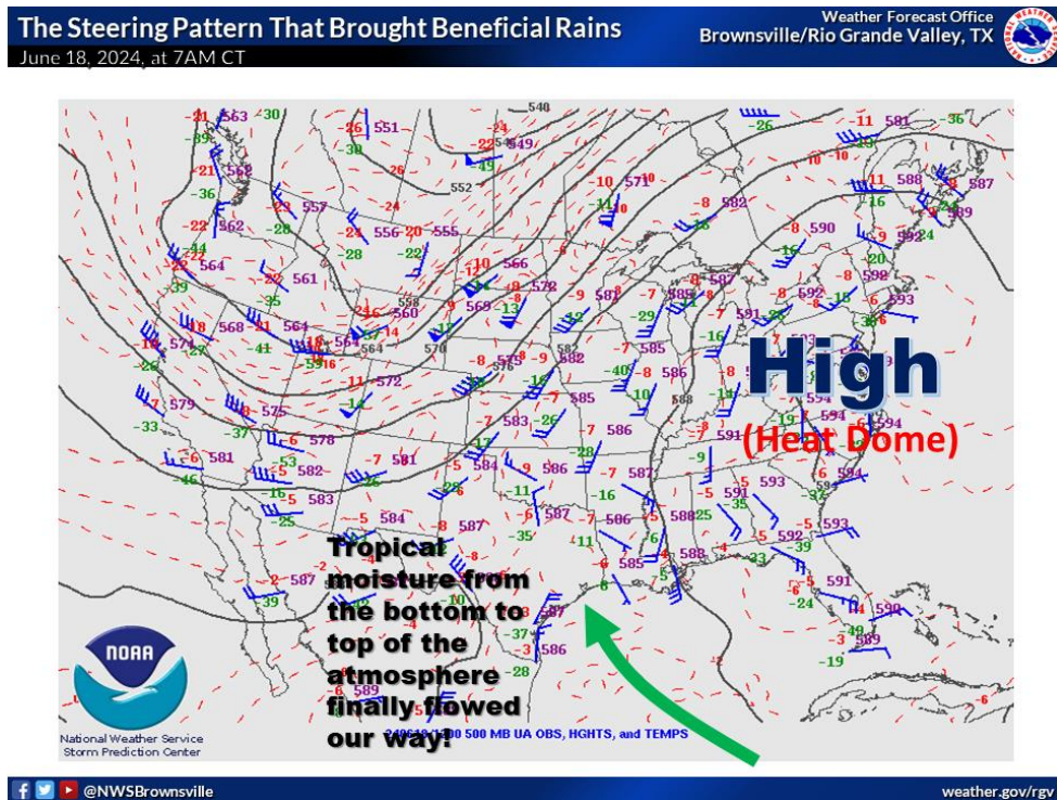
Figure 2. Steering pattern at 500 mb (around 18,000 feet) clearly showing a shift to full-atmospheric flow from the southeast ahead of the wave that would become Tropical storm Alberto on the 19 th .
