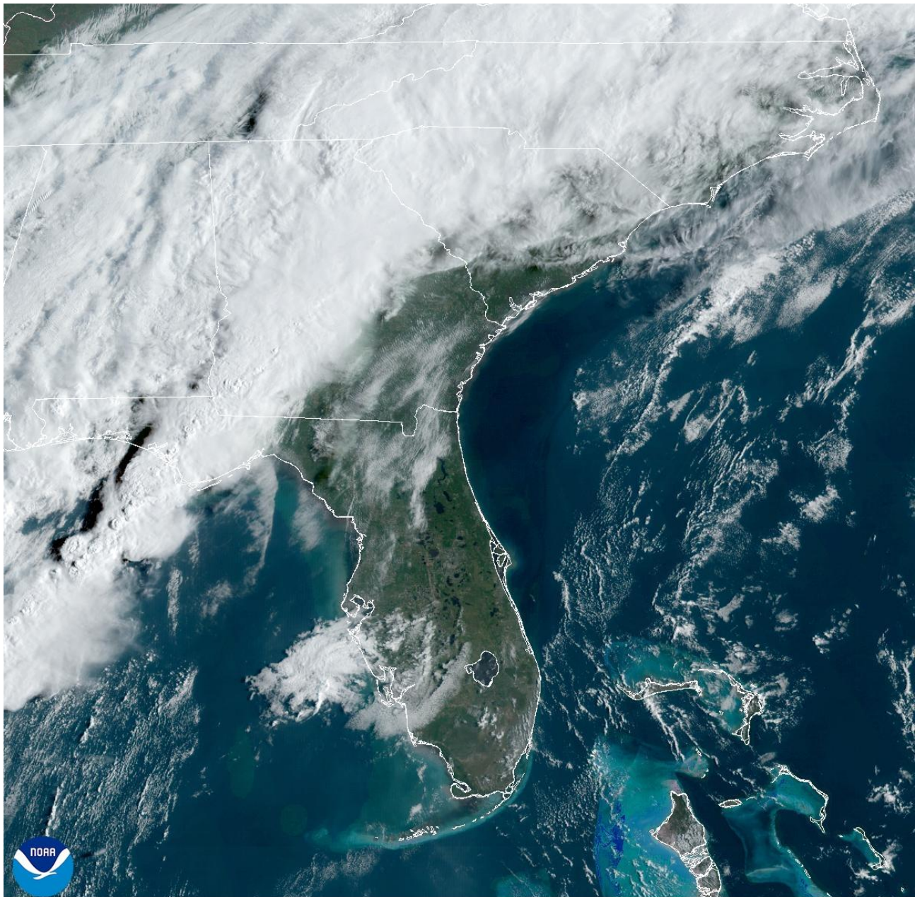
07 Apr 2025 13:06Z - NOAA/NESDIS/STAR - GOES-East - GEOCOLOR Composite - SE
