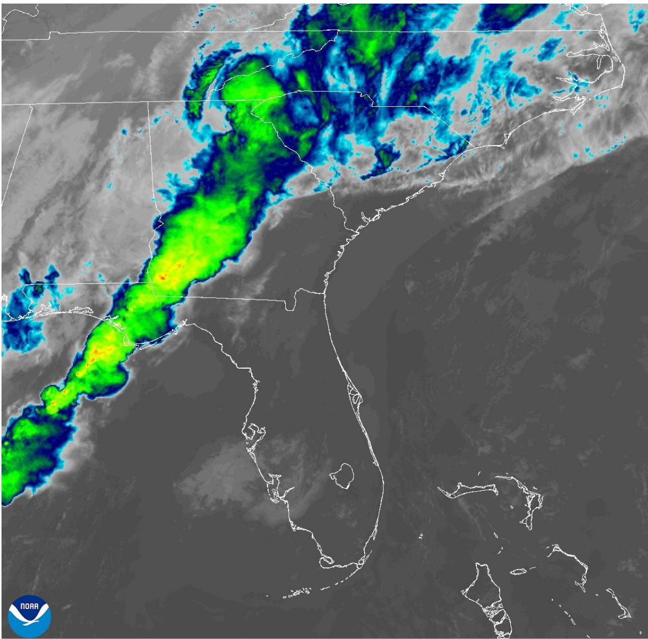
07 Apr 2025 13:01Z - NOAA/NESDIS/STAR - GOES-East - Band 13 - SE
