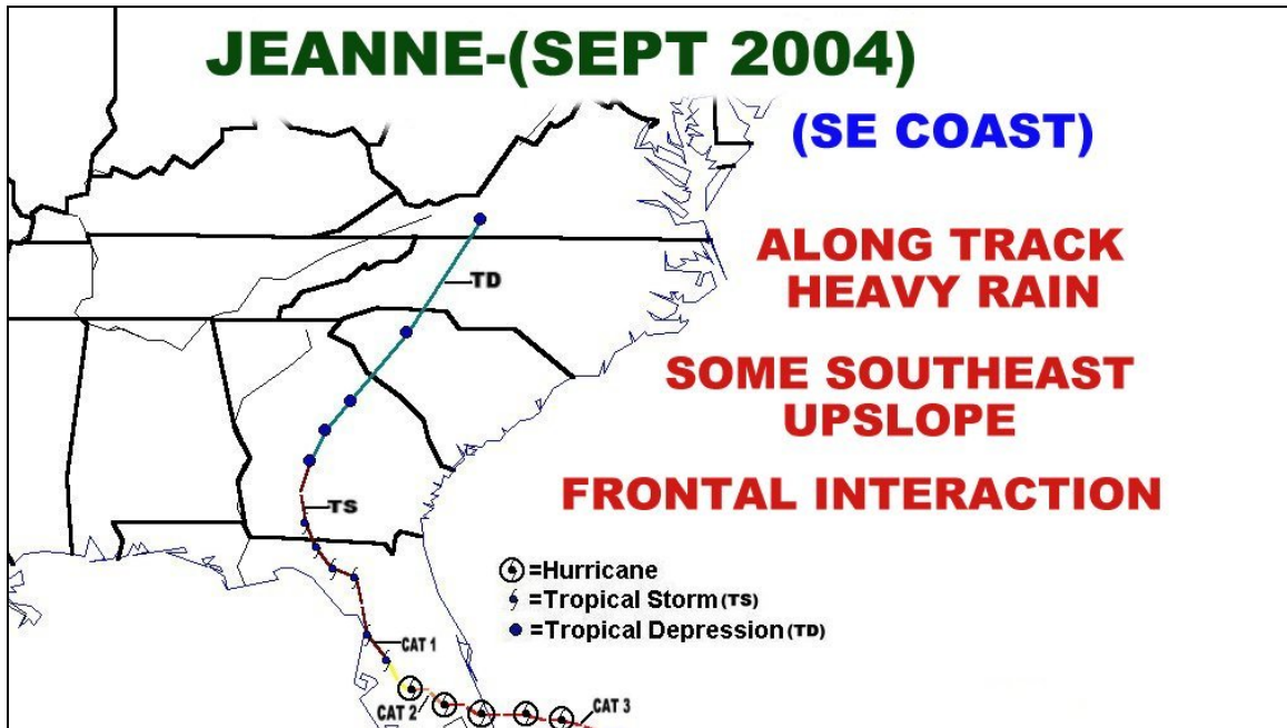
Fig. A-156: September 27-28, 2004. JEANNE .
