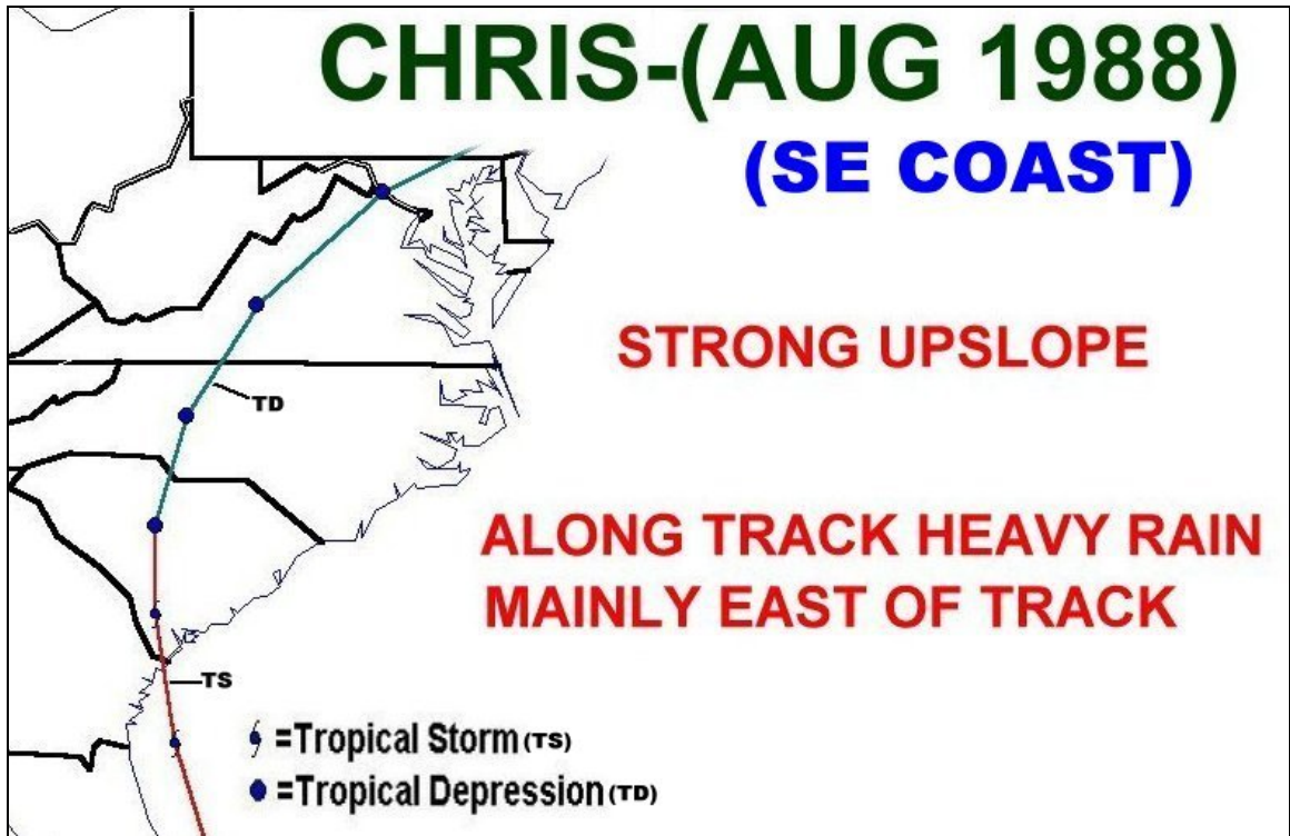
Fig. A-96: August 28-29, 1988. CHRIS .
