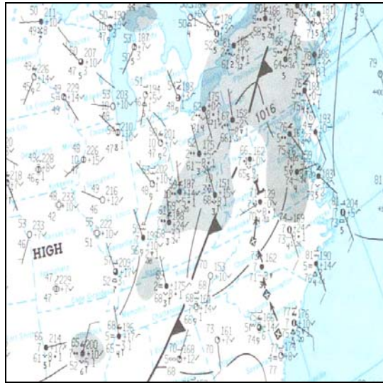
Fig. A-99: Observed standard station plot (4 mb contours), precip. (shaded), 12 UTC, August 29, 1988.
