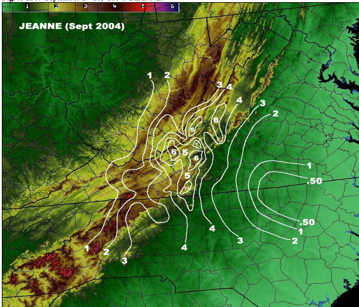
Fig. A-157: Jeanne rainfall in inches (white contours), Sept. 28, 2004, overlaid on terrain (k ft).
