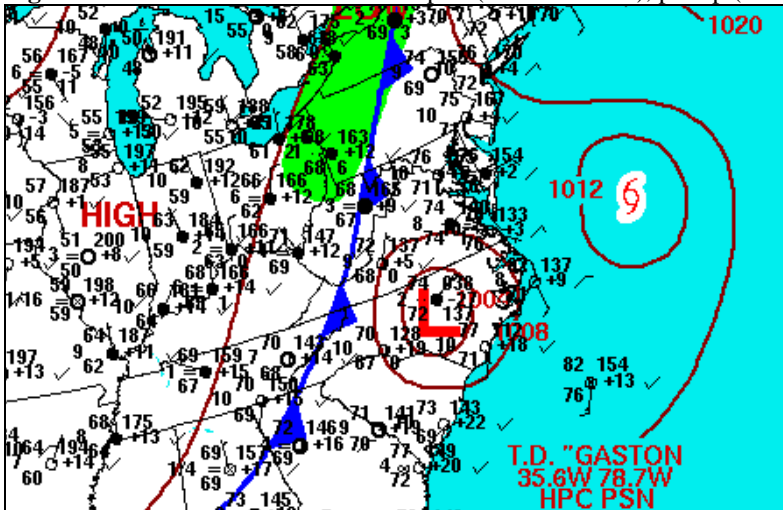
Fig. A-144: Observed standard station plot (4 mb contours), precip (shaded), 12 UTC, August 30, 2004.
