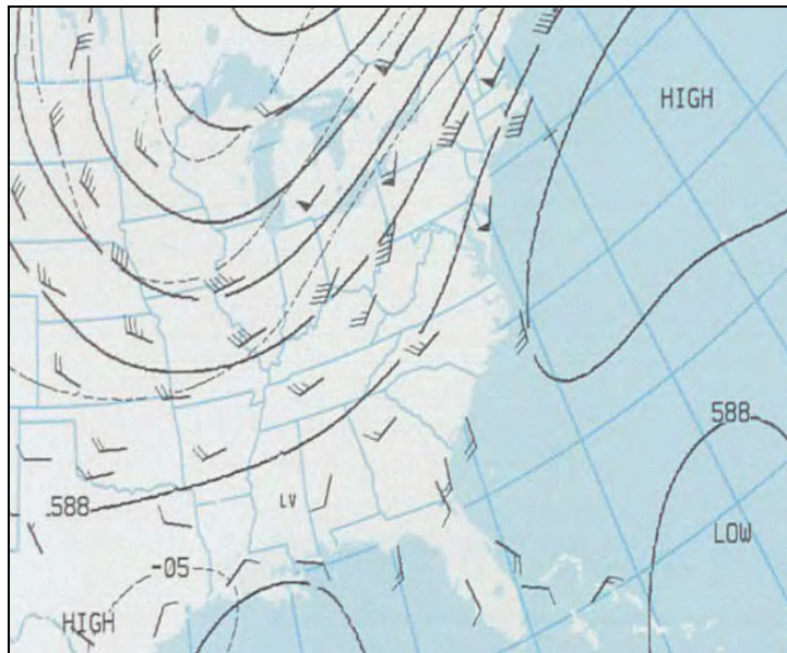
Fig. A-100: Observed 500 mb chart (60 m contours), winds (kts), temperatures (C), 12 UTC, August 29, 1988.
