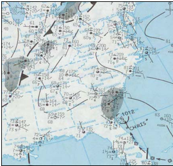
Fig. A-98: Observed standard station plot (4 mb contours), precipitation (shaded), 12 UTC, August 28, 1988.
