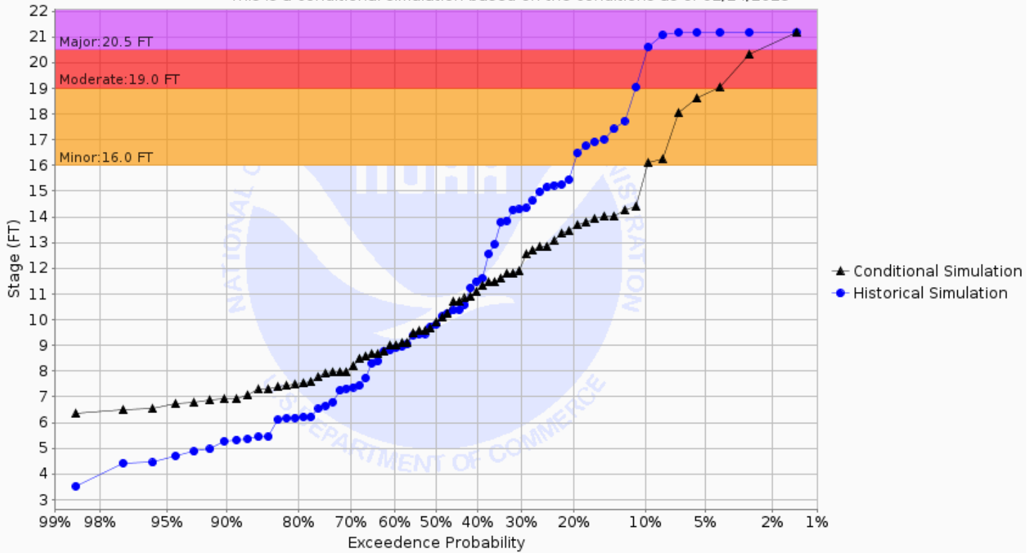
Chance of Exceeding River Stage at Sheyenne River at Kindred 2SE (KNDN8) Forecast for the period 03/03/2025 - 06/01/2025 This is a conditional simulation based on the conditions as of 02/24/2025
